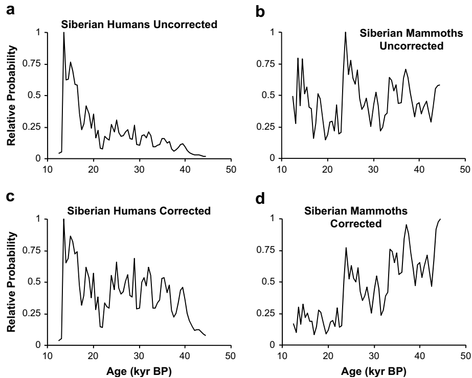
Fig. 5. Temporal frequency distributions of Siberian humans and mammoths from 45 to 12 kyr BP before and after correction with the volcanic model of taphonomic bias. Data from Ugan and Byers (2007). (a) Siberian humans uncorrected. (b) Siberian mammoths uncorrected. (c) Siberian humans corrected. (d) Siberian mammoths corrected.
