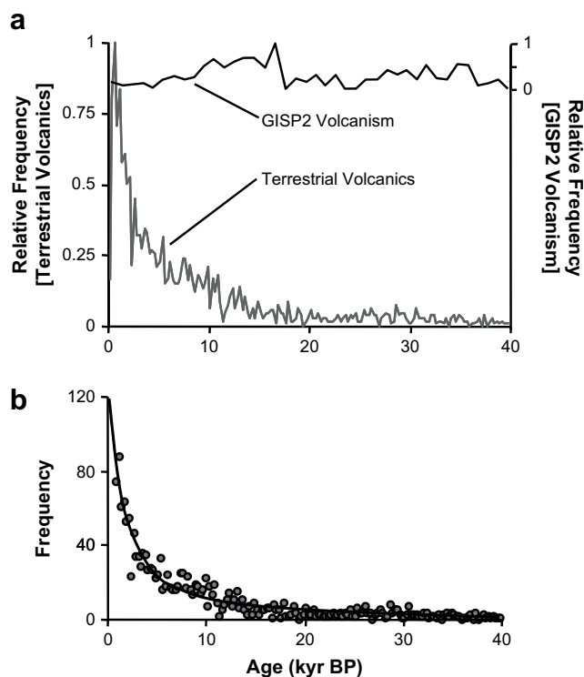
Fig. 1. (a) Temporal frequency distribution of radiocarbon dated terrestrial volcanic deposits (data from Bryson et al., 2006) compared to the frequency distribution of major volcanic eruptions evident in the GISP2 ice core, Greenland (data from Zielinski et al., 1994). (b) A regression model of taphonomic bias derived from the Bryson et al. (2006) database. The fit line is: \text{freq} = 5.726442 \times 10^6(\text{age} + 2176.4)^{-1.3925309} .
