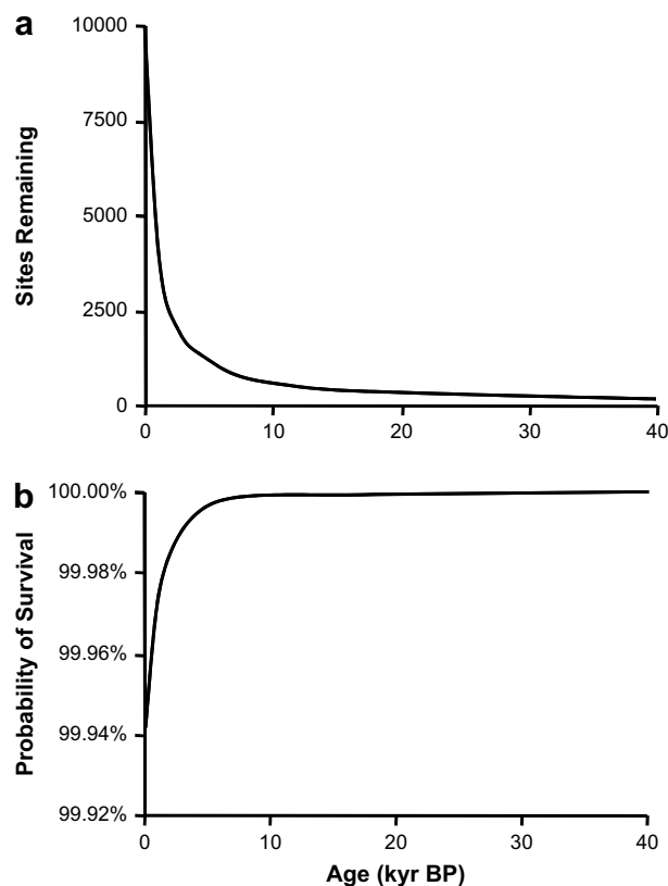
Fig. 2. Properties of the empirically derived model of taphonomic bias. (a) The predicted loss of archaeological sites over time assuming 10,000 sites at time zero. (b) The annual likelihood of survival ( 1 - \lambda ) as a function of site age.
