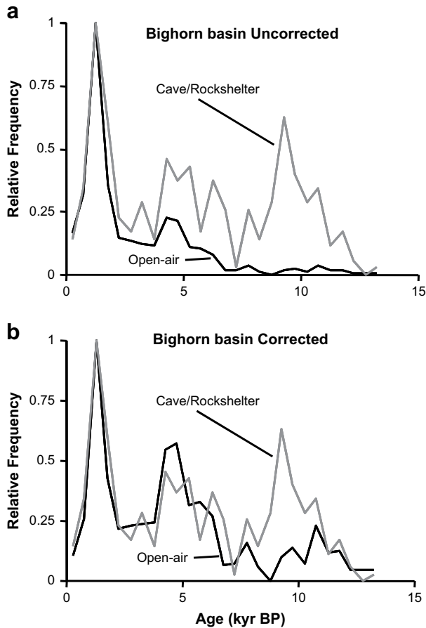
Fig. 3. Temporal frequency distributions of ^{14}\text{C} dates from open-air and rockshelter sites in the Bighorn basin of Wyoming. (a) Open-air frequencies uncorrected for taphonomic bias. (b) Open-air frequencies corrected for taphonomic bias using the volcanic correction.
