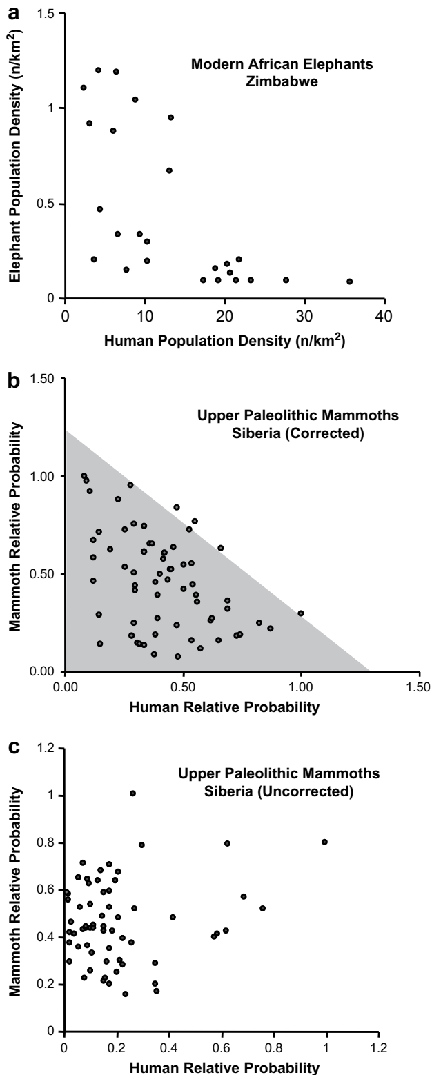
Fig. 6. (a) Human vs. African elephant crude population density in the Sebungwe region of northwestern Zimbabwe. Figure redrafted from Hoare and du Toit (1999: Fig. 3). (b) Human vs. woolly mammoth population density from 44.5 to 13.5 kyr BP inferred from relative probabilities after correction for taphonomic bias as shown in Fig. 5c and d. The upper bound of the gray triangle was determined by linear regression of the mean human relative probability vs. maximum mammoth relative probability for five intervals of 0.2 unit width of the x-axis. Human vs. woolly mammoth population density from 44.5 to 13.5 kyr BP inferred from relative probabilities before correction for taphonomic bias as shown in Fig. 5a and b.
