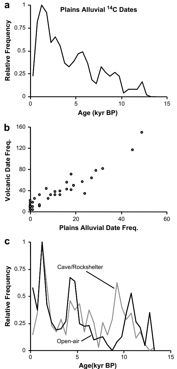
Fig. 4. (a) Temporal frequency distributions of ^{14}\text{C} dates from alluvial geologic contexts in the Great Plains and adjacent regions (data from Baker et al., 2000; Mandel, 1995; Martin, 1992; Meyer et al., 1995). (b) The frequency of radiocarbon dates in 500-year time intervals from 1000 to 20,000 BP in Great Plains alluvial contexts vs. the Bryson et al. (2006) terrestrial volcanism database. (c) Temporal frequency distributions of ^{14}\text{C} dates from open-air and rockshelter sites in the Bighorn basin of Wyoming open-air frequencies were corrected for taphonomic bias using the database of local geologic dates.
