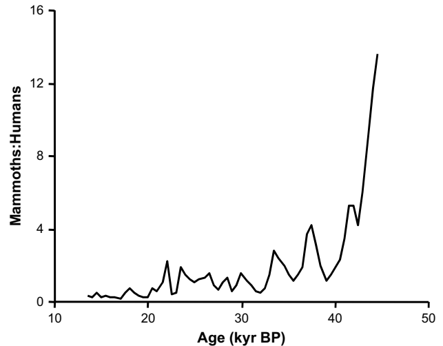
Fig. 7. The ratio of mammoth to human population density in Siberia from 44.5 to 13.5 kyr BP based on the temporal frequency distributions shown in Fig. 5a and b.
